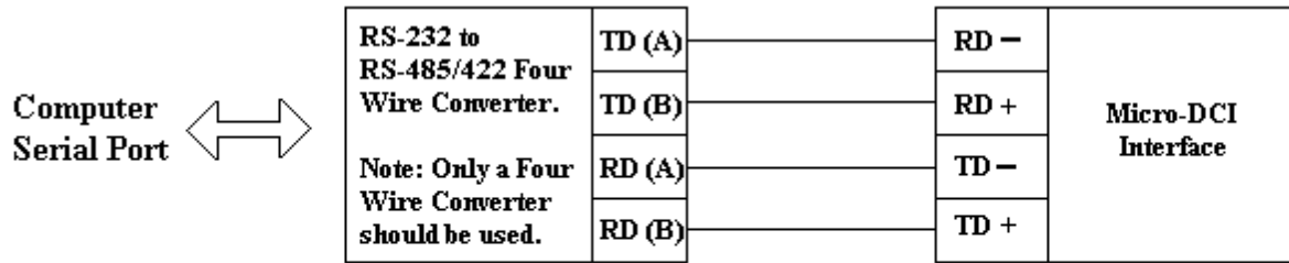
Figure 2. Data Link Port Cable Connection
