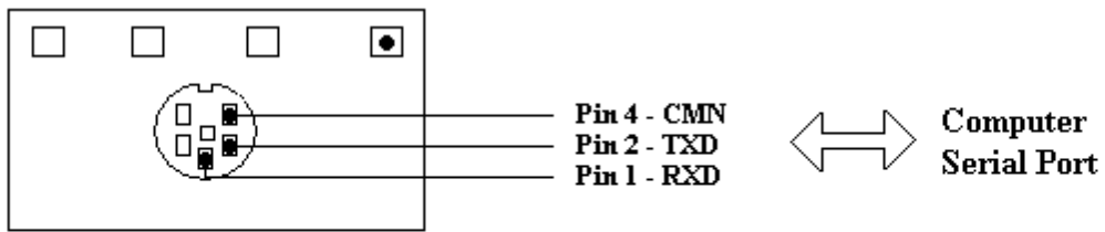
Figure 1. Configuration Port Cable Connection
